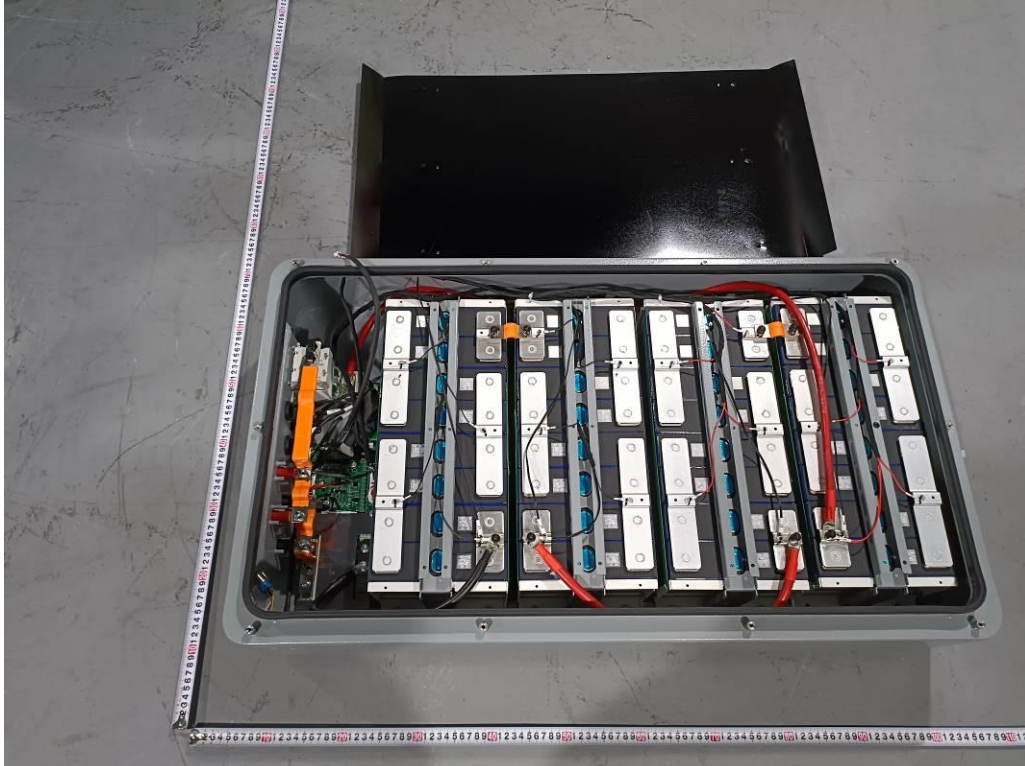
Figure 7 Internal view
