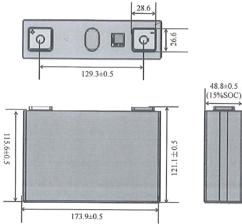
Figure 3 Cell
