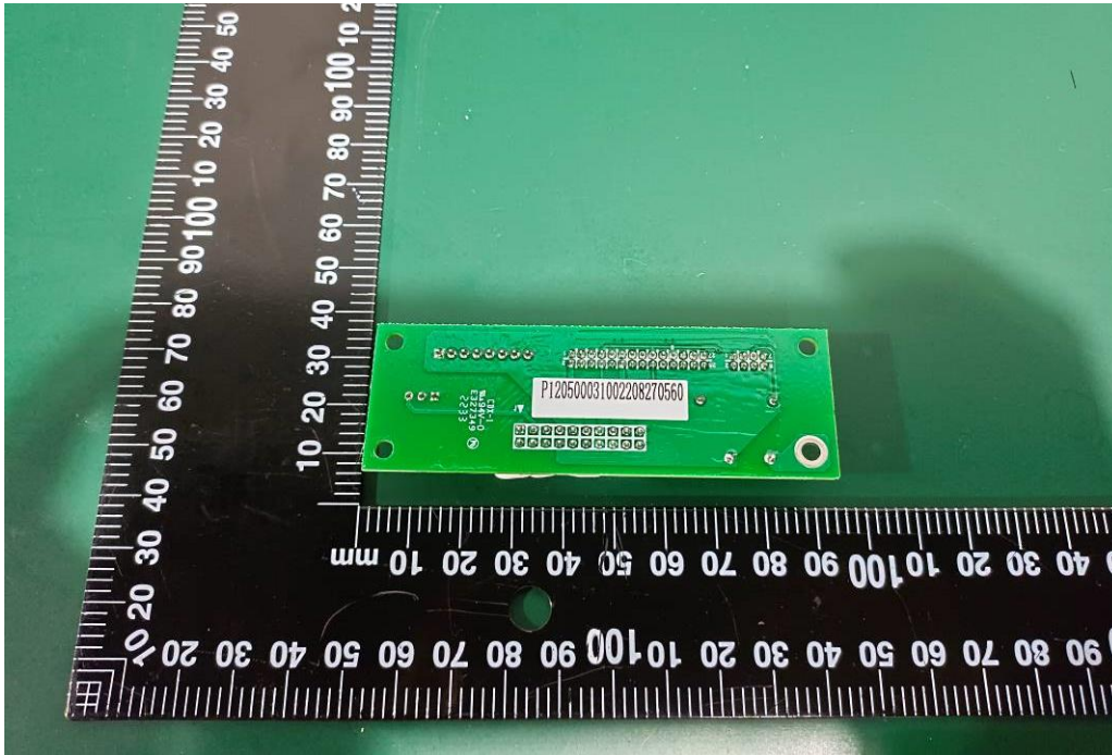
Figure 13 Bottom view of COMM board
