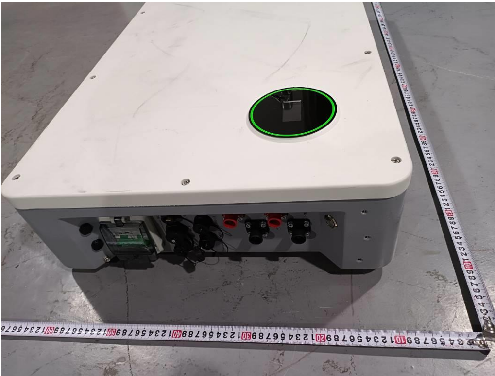
Figure 4 Side view
