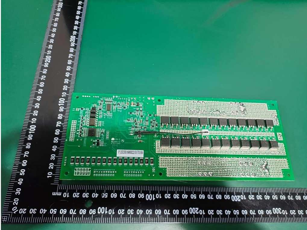
Figure 11 Bottom view of BMS board
