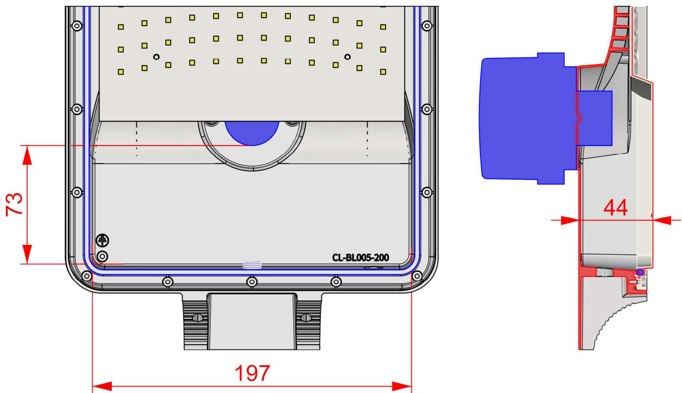
驱动电源尺寸：W197mm*L73mm*H44mm
