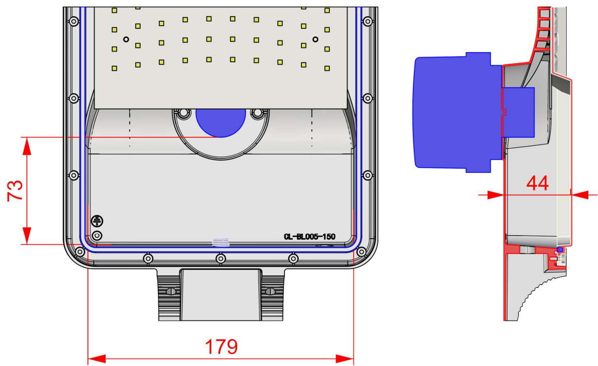
驱动电源尺寸：W179mm*L73mm*H44mm
