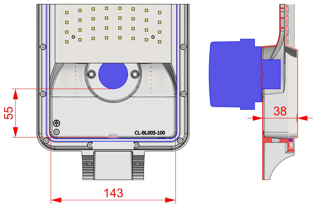
驱动电源尺寸：W143mm*L55mm*H38mm
