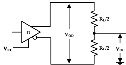
Fig 2 Driver DC test load
