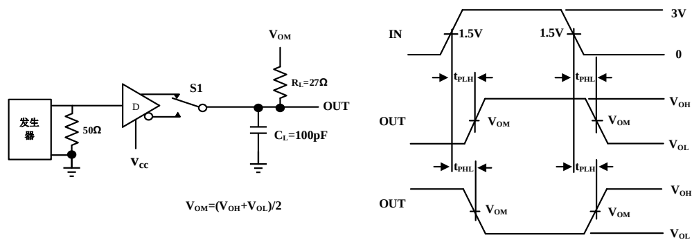
Fig 4 Driver propagation times
