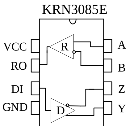
Fig 1 KRN3085E Pin Configuration
