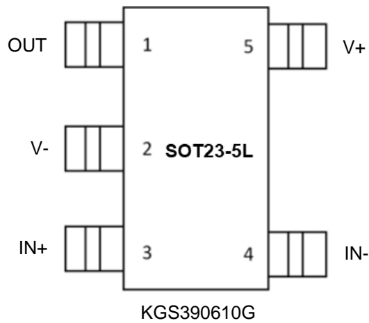
Figure 3 KGS390610G/N Pinouts
