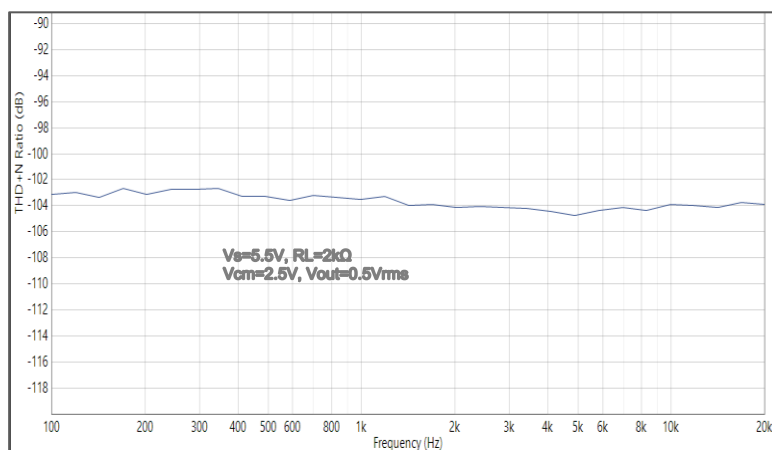
Figure 7 THD+N vs Frequency
